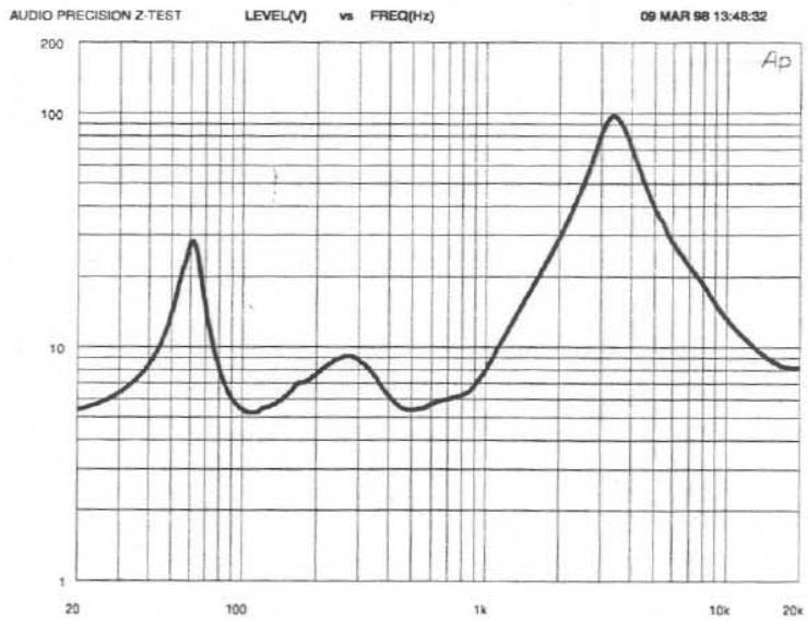
Figure 6b — Full-Range Impedance Curve (closed ports)
